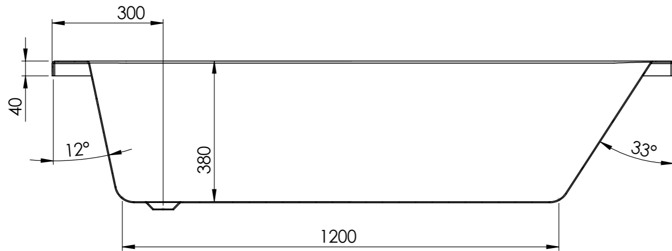
SECTION C-C SCALE 1 : 10
